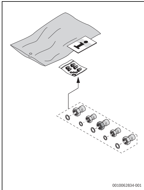
3 Pipe Kit, 7 736 902 029
