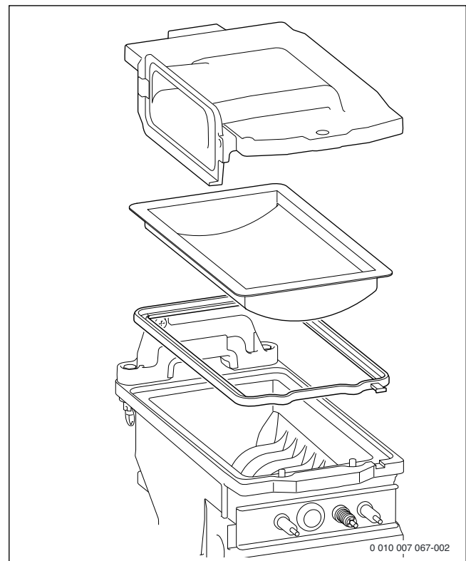
Obr. 94 Hořák
