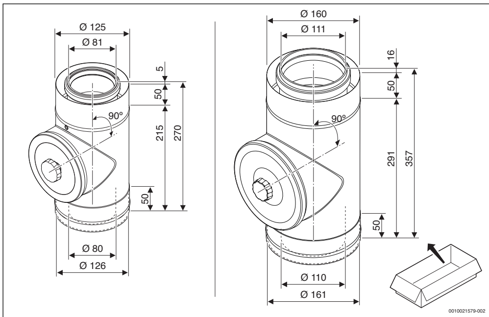
1 \text{Ø} 80/125 \text{ mm: } 7738112704, \text{Ø} 110/160 \text{ mm: } 7738113148
