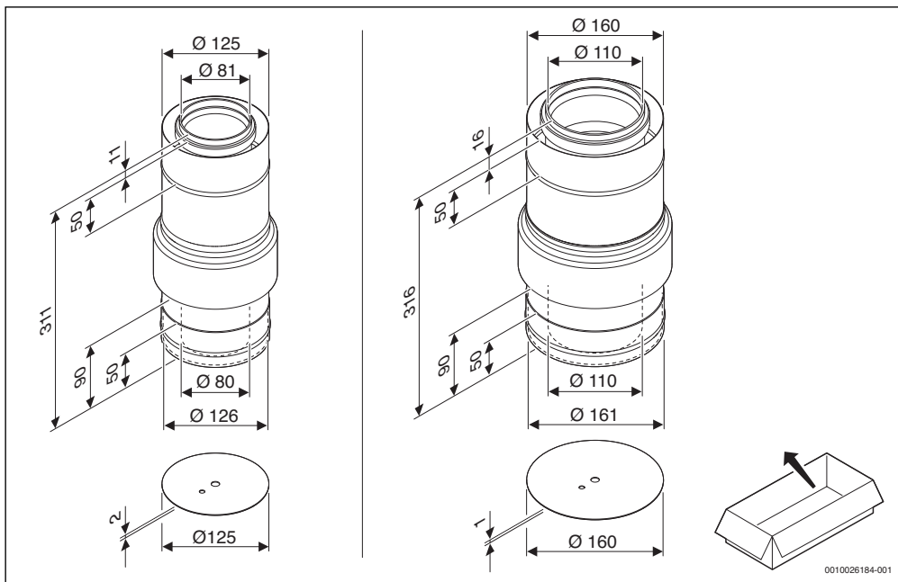
1 Ø 80 mm: 7738112705, Ø 110 mm: 7738113147
