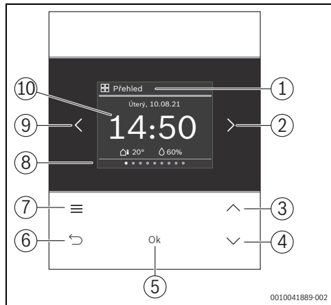
Obr. 1 Logamatic RC220
