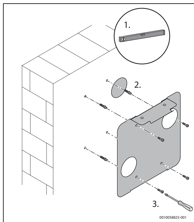
Afb. 34 Monteer de console
